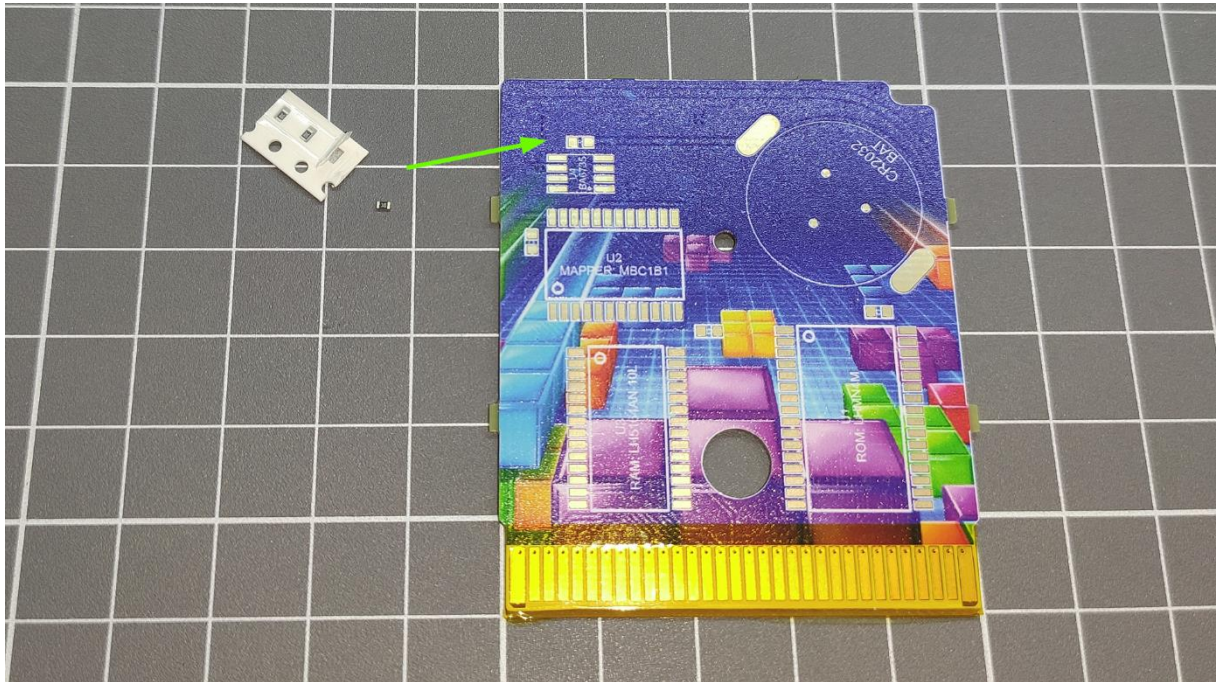
Resistor installation (Board version 1.1)
